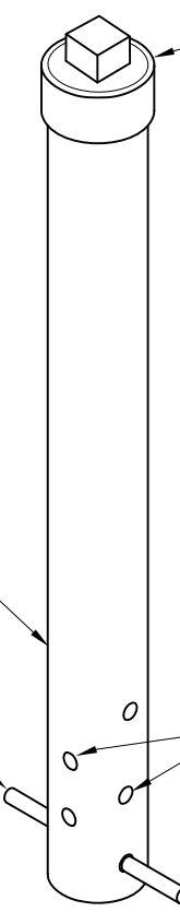
OBSERVATION PIPE DETAIL N.T.S.
